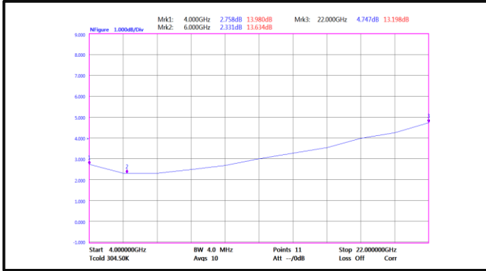
Noise Figure(4-22GHz)
