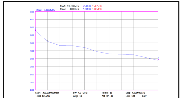
Noise Figure(0.2-4GHz)
