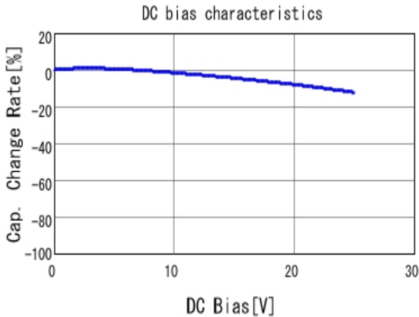
■ GRM21BR71E104KA01 C-DC bias capchange, 25.0degC, AC1.
