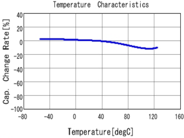
■ GRM21BR71E104KA01 C-Temp. capchange, DC0.0V, AC1.0V r m
