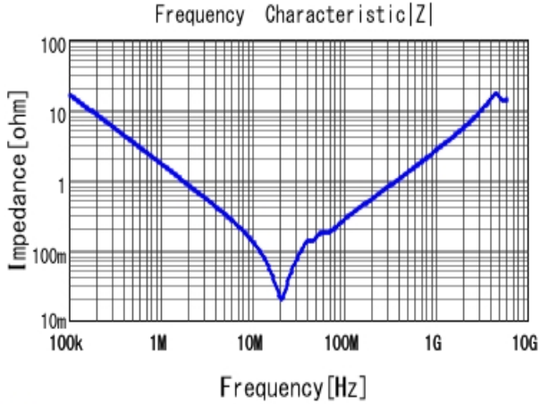
■ GRM21BR71E104KA01 |Z| DCOV, 25degC
