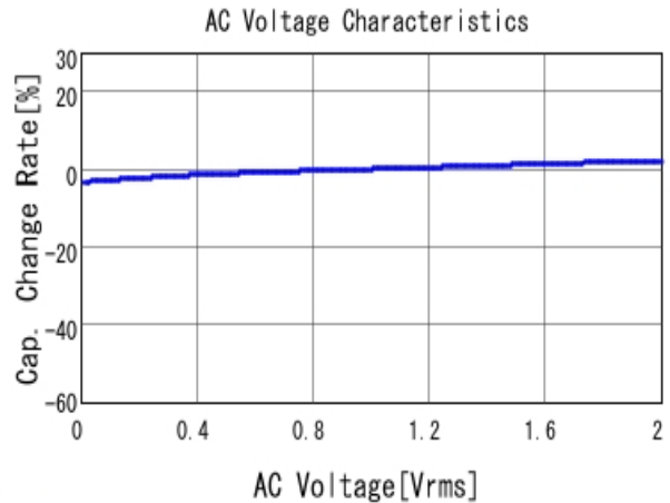
■ GRM21BR71E104KA01 C-AC Voltage capchange, DCOV, 25.0d
