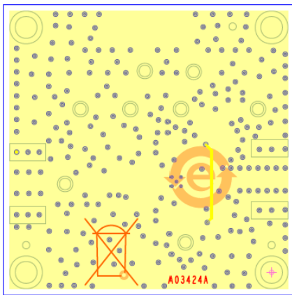
Figure 65. ADL5906 Evaluation Board Layout, Bottom Side
