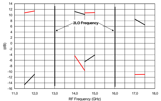
Typical on wafer measurement: Conversion Gain & Image suppression @ IF=1& 1.5GHz
