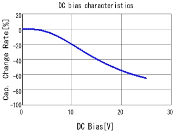
■ GRM219R71E105KA88 C-DC bias capchange, 25.0degC, AC1.
