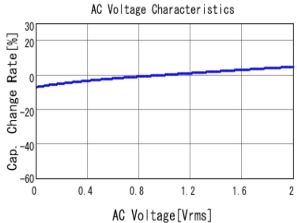
■ GRM219R71E105KA88 C-AC Voltage capchange, DCOV, 25.0d
