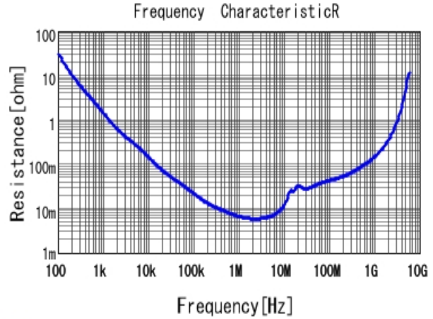
■ GRM219R71E105KA88 R DCOV, 25degC
