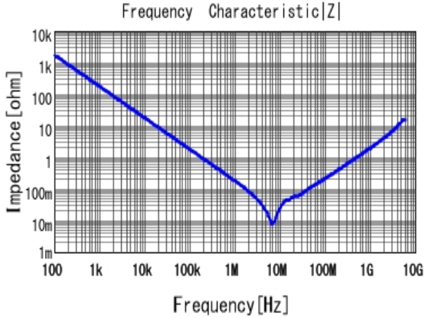
■ GRM219R71E105KA88 |Z| DCOV, 25degC
