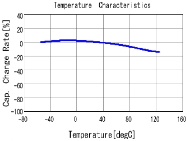
■ GRM219R71E105KA88 C-Temp. capchange, DC0.0V, AC1.0V r m
