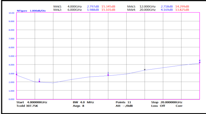
Noise Figure(4-20GHz)
