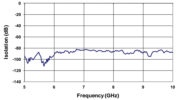
Isolation (5-10 GHz)
