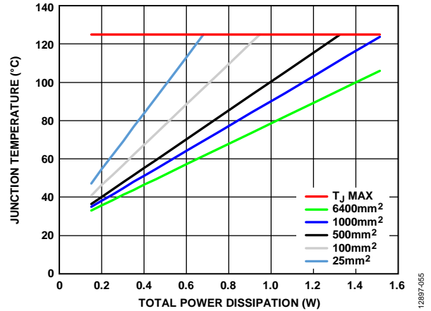
Figure 50. Junction Temperature vs. Total Power Dissipation, T_A = 25^\circ\text{C}
