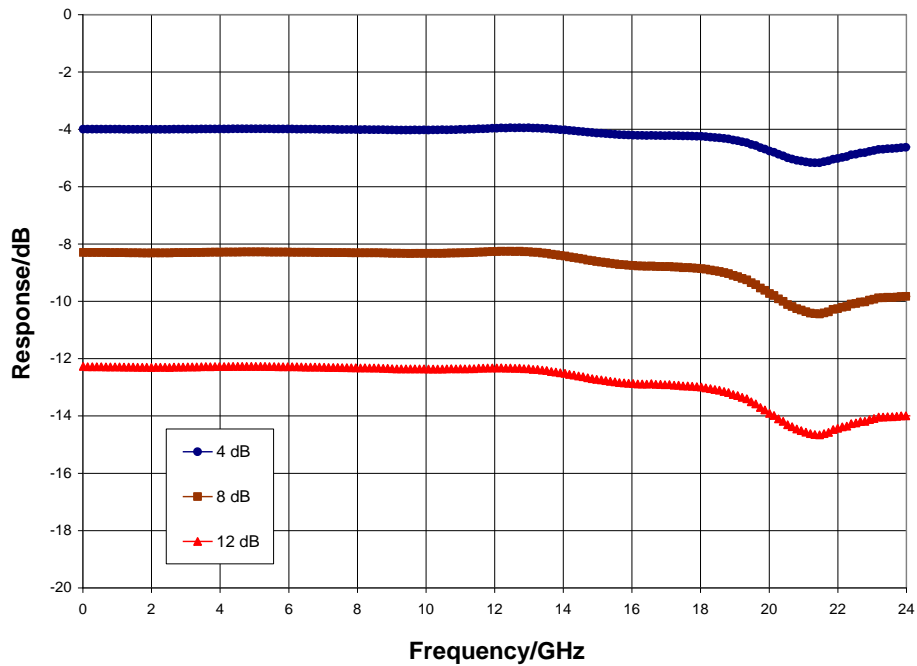
Normalized Attenuation (all states), T_A = 25\text{ }^\circ\text{C}
