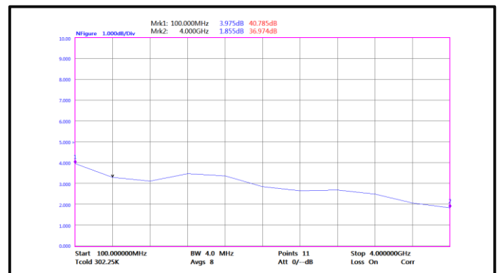
Noise Figure(0.1GHz-4GHz)
