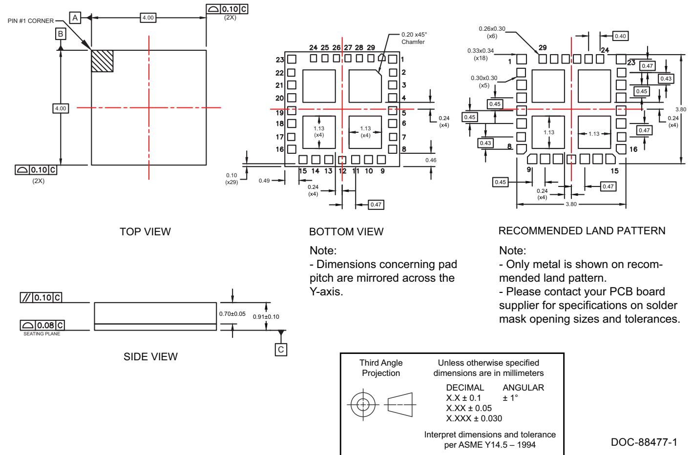
Figure 24 • Package Mechanical Drawing for 29-lead 4 × 4 × 0.91 mm LGA
