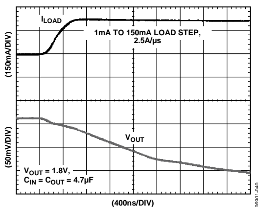
Figure 29. Output Transient Response, C_{OUT} = 4.7\ \mu\text{F}
