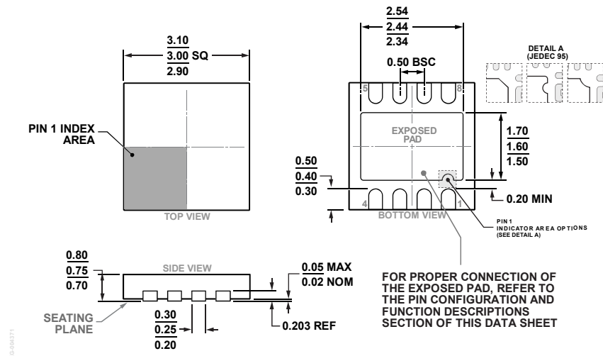
Figure 70. 8-Lead Lead Frame Chip Scale Package [LFCSP] 3 mm × 3 mm Body and 0.75 mm Package Height (CP-8-21) Dimensions shown in millimeters
