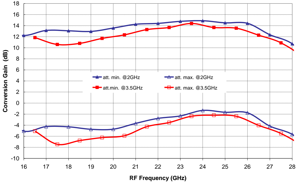
Conversion Gain in Supradyne Mode versus RF Frequency & IF F_{RF} = 2 \times F_{LO} + F_{IF} , GCx = -1.5V & 0V Board losses de-embedded (result given on package access planes)
