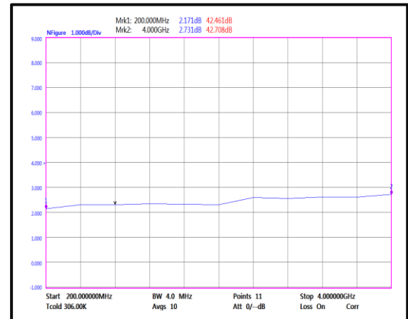
Noise Figure(0.2GHz-4GHz)
