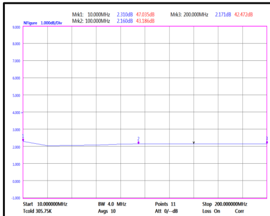
Noise Figure(0.01GHz-0.2GHz)
