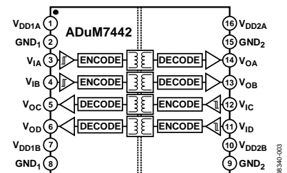
Figure 3. ADuM7442
