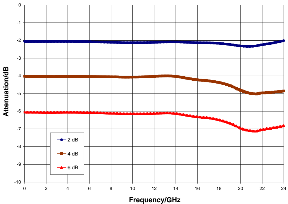
Normalized Attenuation (all states), T A = 25 °C
