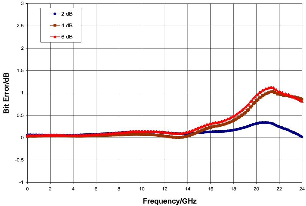
Bit Error versus Frequency, T_A = 25\text{ }^\circ\text{C}
