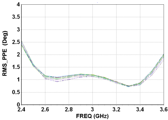
RMS phase error versus frequency for 15 chips
