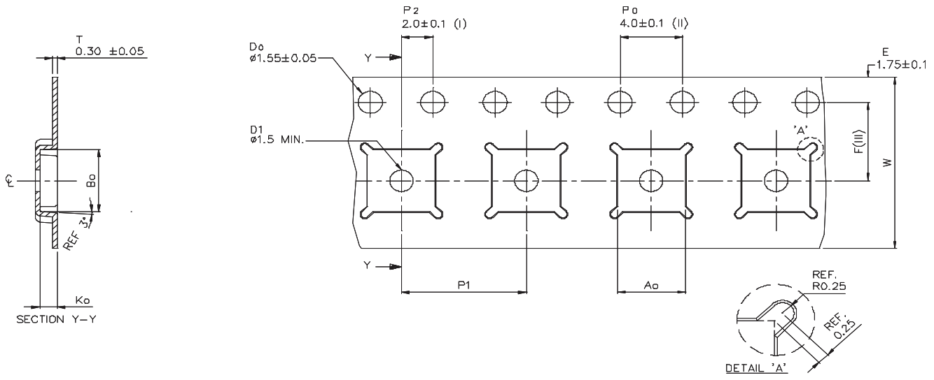
Figure 20 • Tape and Reel Drawing
