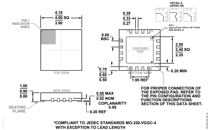
Figure 26. 16-Lead Lead Frame Chip Scale Package [LFCSP] 4 mm × 4 mm Body and 0.90 mm Package Height (CP-16-40) Dimensions shown in millimeters
