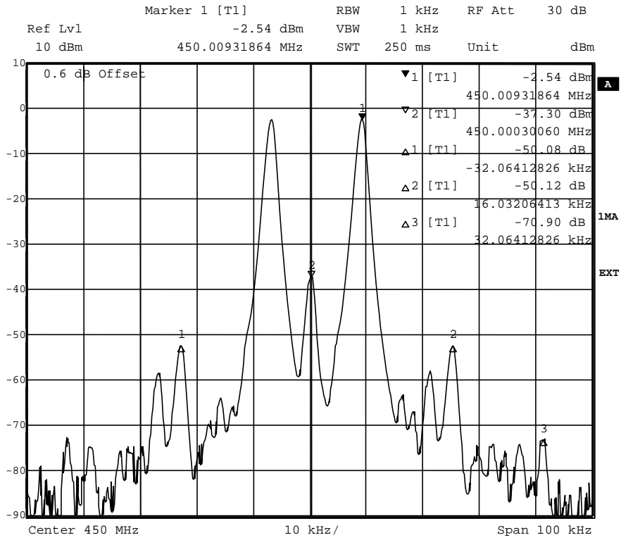
Figure 8 +3dBm PEP Output, two-tone input at 450MHz
