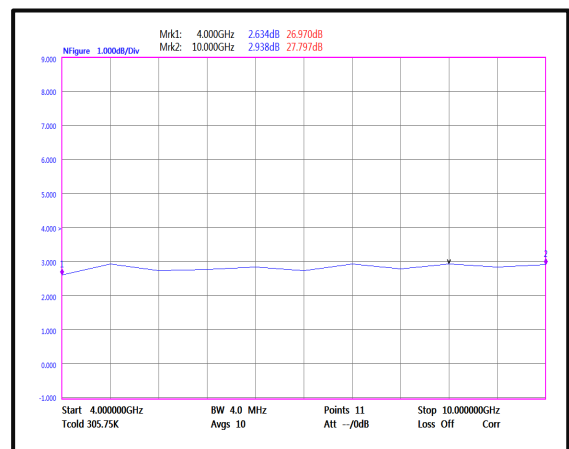
Noise Figure(4-10GHz)
